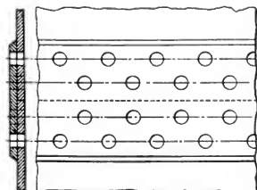
Figs. 323-324. Double Riveted Butt Joint with One Welt.
